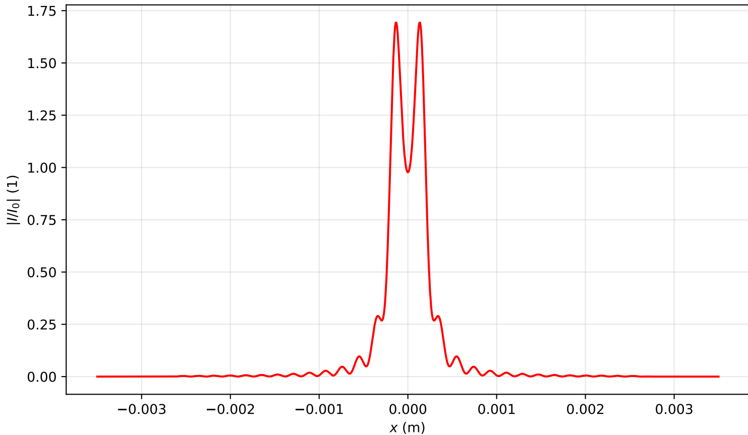
Intensity profile I(x, y = 0, z = 0.159)/I_0 , P_{in}=4.0P_{cr} , artificial time
